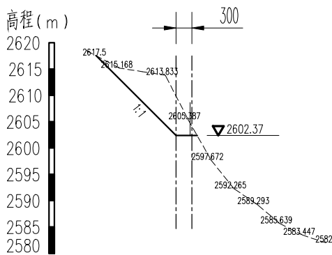
KA9-0+071.75 1: 1000
